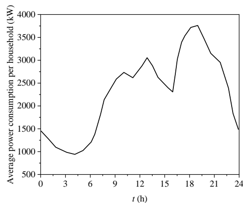
Fig. 2. Typical Daily Load Curve of the Distribution Network
